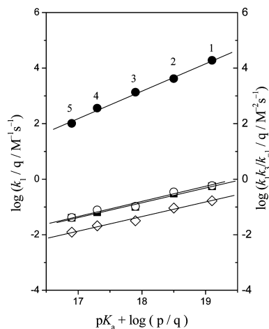
Figure 4. Brønsted-type plots for reactions of 1a–d with cyclic secondary amines 1–5 in MeCN at 25.0 \pm 0.1 °C: 1a (●, \beta_{\text{nuc}} = 1.00 ), 1b (■, \beta_{\text{nuc}} = 0.53 ), 1c (○, \beta_{\text{nuc}} = 0.53 ), 1d (◇, \beta_{\text{nuc}} = 0.52 ). Note that the k_1 k_3 / k_{-1} values (taken from Table 2) for the reaction of 1a are used in the Brønsted-type correlation with q = 4 for piperazine. The assignment of numbers is given in Tables 1 and 2.
