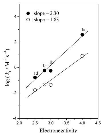
Figure 5. Plots of \log k_1 vs electronegativity of X for reactions of 1a–d with piperidine in MeCN (●) and H 2 O (○) at 25.0 \pm 0.1 °C. Note that the k_1 values for the reaction of 1a in MeCN are used in the correlation.
