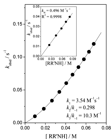
Figure 1. Plots of k_{\text{obsd}} vs [\text{RR}'\text{NH}] for the reaction of 1a with diethylamine in MeCN and in \text{H}_2\text{O} (inset) at 25.0 \pm 0.1 °C. The solid line for the reaction in MeCN was calculated by eq 1.
